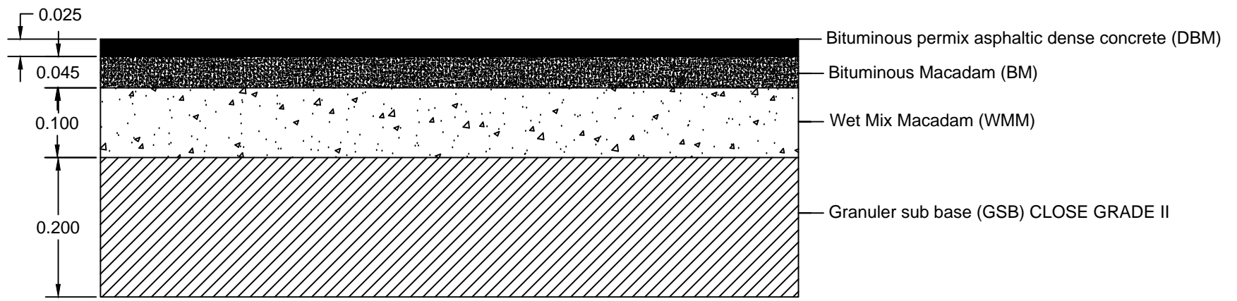
TYPICAL CROSS SECTION OF RESTORATION OF TRENCHES FOR BITUMINOUS ROAD ( INCLUDING TACK COAT ON TOP OF BM AND DBM
