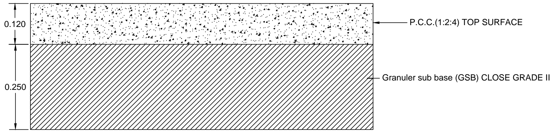
TYPICAL CROSS SECTION OF RESTORATION OF TRENCHES FOR CONCRETE SURFACE
