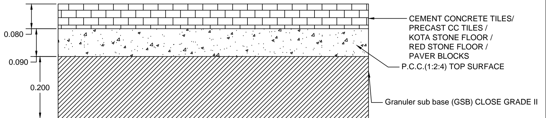
TYPICAL CROSS SECTION OF RESTORATION OF TRENCHES FORCEMENT CEMENT CONCRETE TILES/PRECAST CC TILES /KOTA STONE FLOOR /RED STONE FLOOR /PAVER BLOCKS
